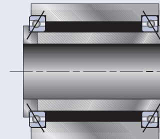
Back-to-back mounting
